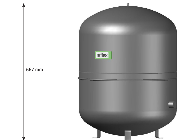
Reflex S 100 litri / 10 bar
